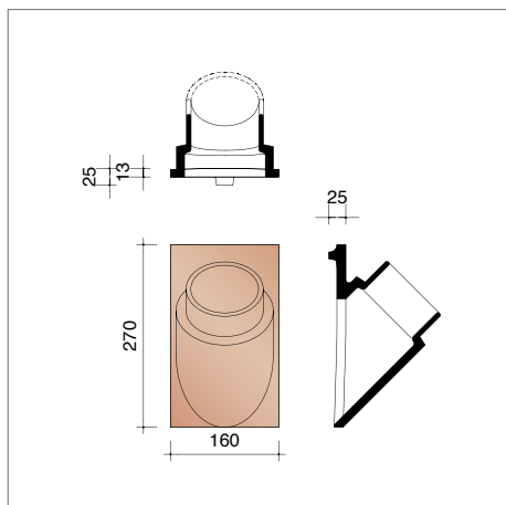
AAR78720 Kokerpan Ø 100 mm
